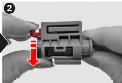
(2) Push the release down
